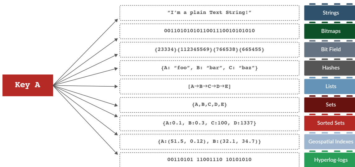
Figure 3. Redis data structures are like building blocks
