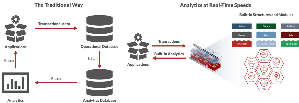
Figure 5. Modern day transactional and analytical scenarios
