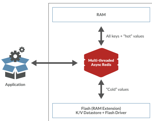
Redis on Flash uses a combination of RAM and Flash memory
