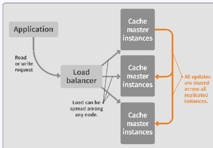
Figure 6-3. Multi-master replication
